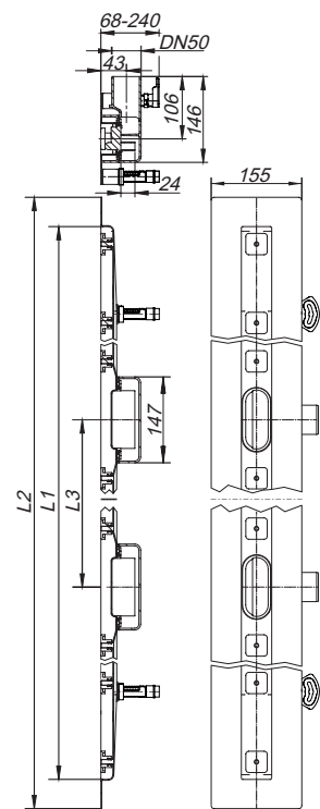
douchegoot CeraLine Nano F Duo 800 – 2000
