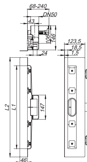
douchegoot CeraLine Nano W 500 – 1200
