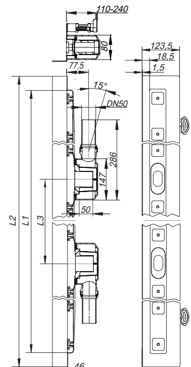
douchegoot CeraLine W Duo 800 – 1200
