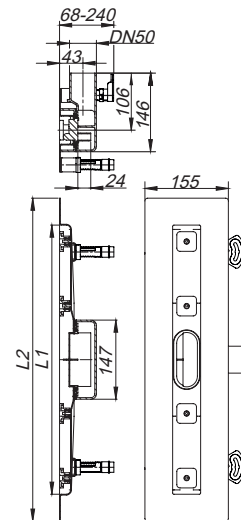
douchegoot CeraLine Nano F 500 – 1200
