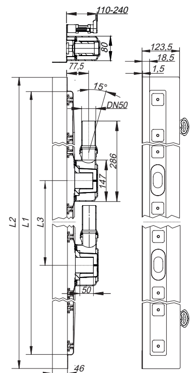
douchegoot CeraLine W Duo 1300 – 2000
